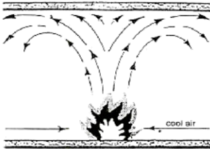
Convection
