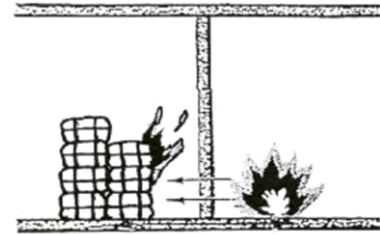
Conduction
