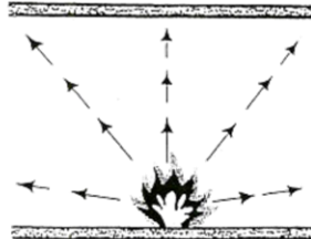
Radiation
