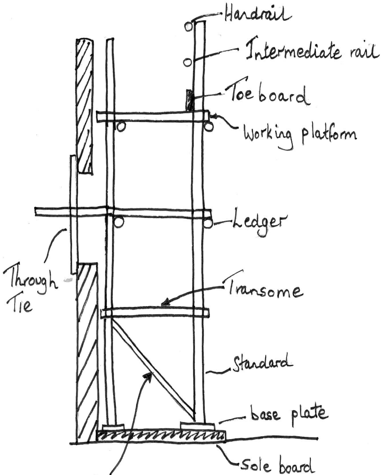
INDEPENDENT TIED SCAFFOLDS
